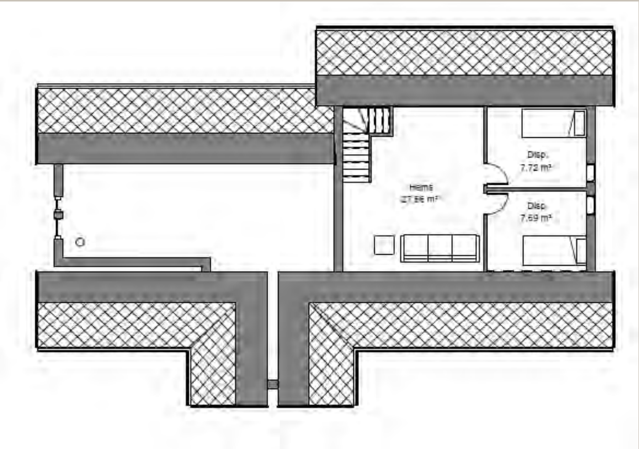
Hemsplan
