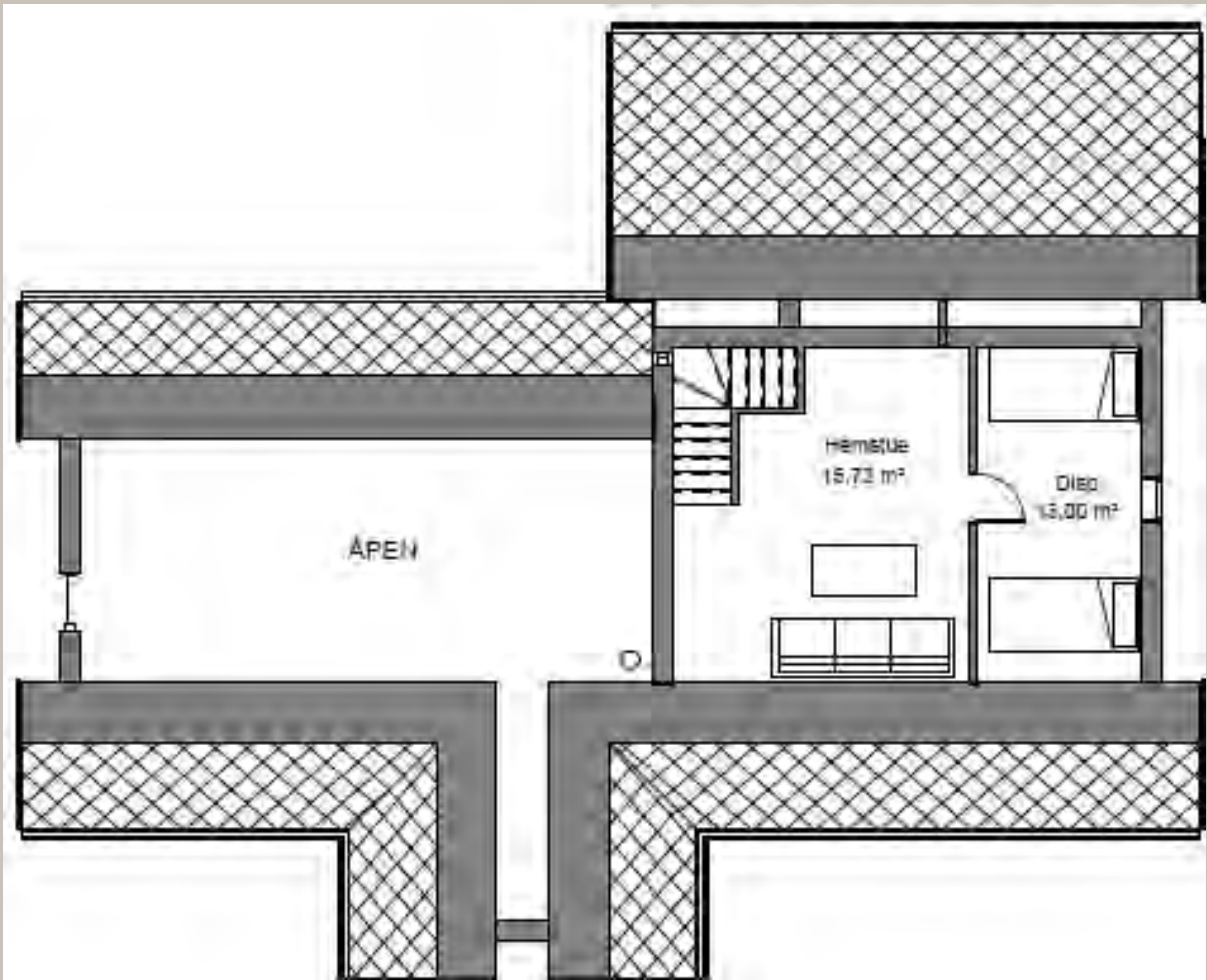
Hemsplan
