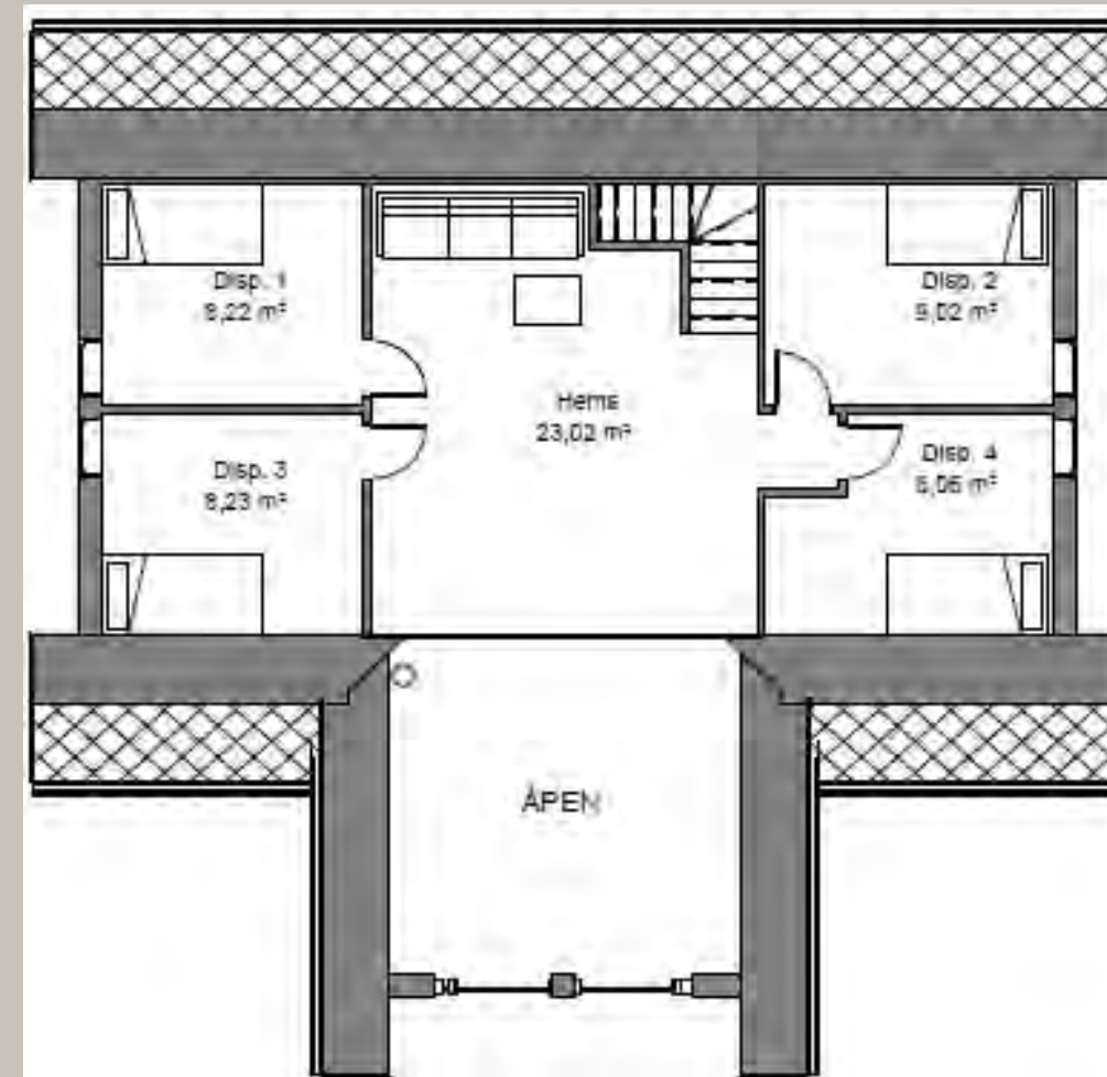
Hemsplan
