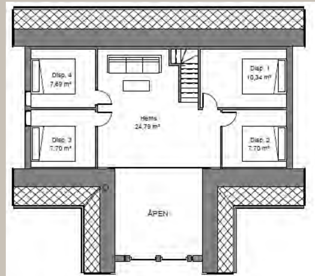
Hemsplan
